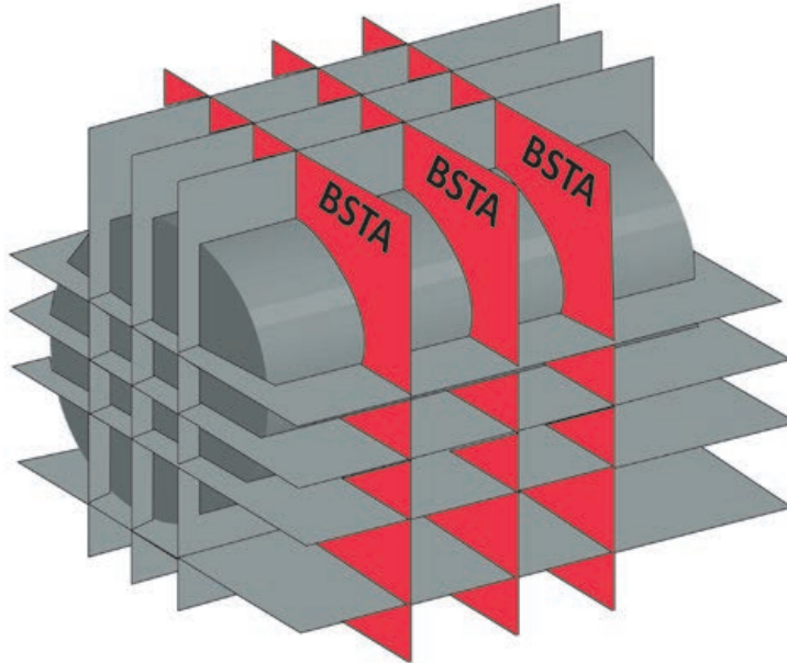
Görsel 5.9: Fuselage station örneği
