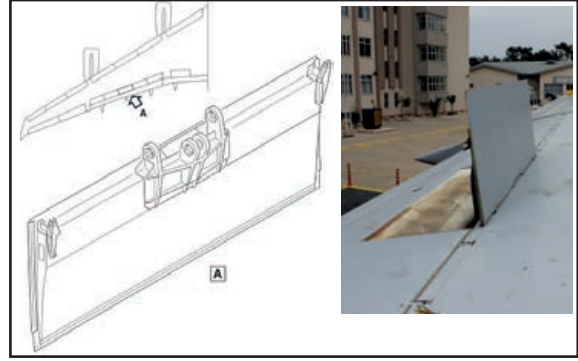
Görsel 6.17: Spoiler
