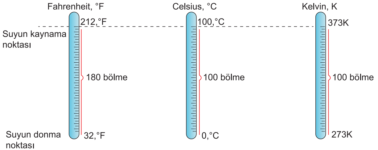
Şekil 3.8: Fahrenheit, Celcius ve Kelvin termometreleri
